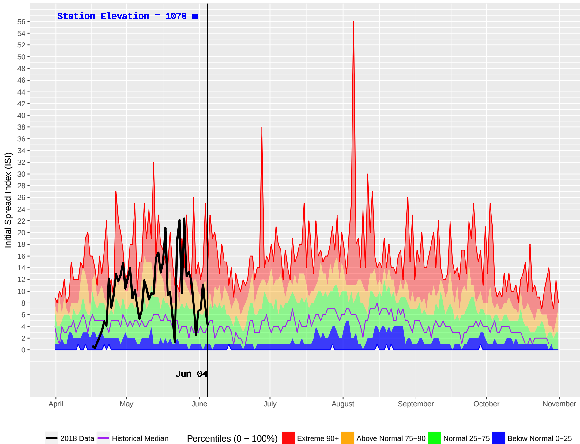
MEADOW LAKE (236) : Historical (1991–2016) and Current (2018) Noon Initial Spread Index (ISI)
