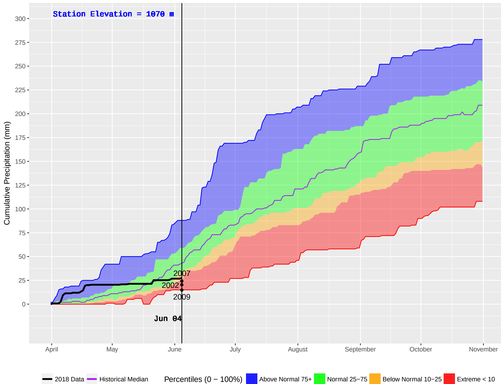
MEADOW LAKE (236) : Historical (1991–2016) and Current (2018) Noon Cumulative Precipitation
