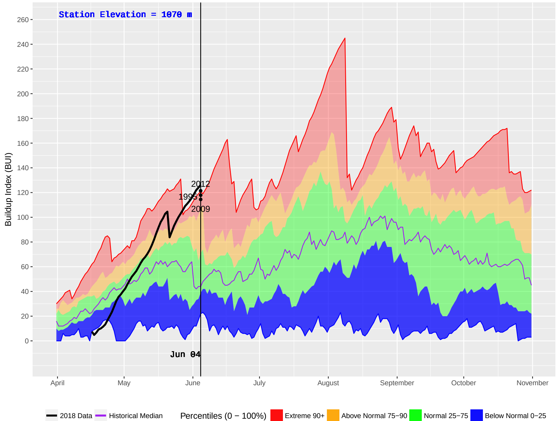
MEADOW LAKE (236) : Historical (1991–2016) and Current (2018) Noon Buildup Index (BUI)
