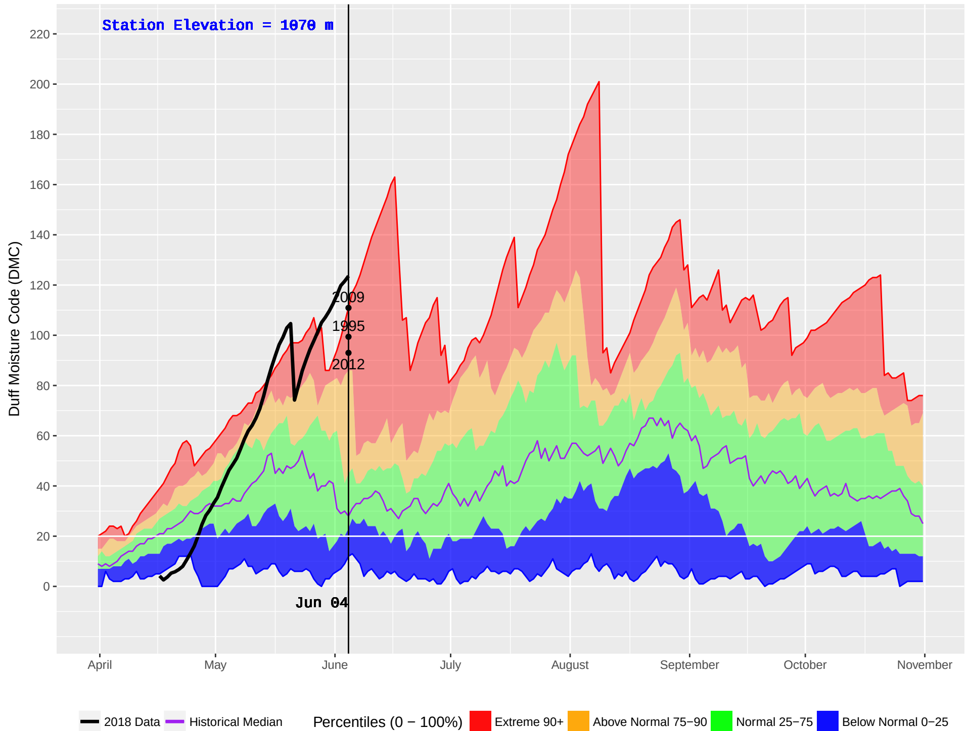
MEADOW LAKE (236) : Historical (1991–2016) and Current (2018) Noon Duff Moisture Code (DMC)
