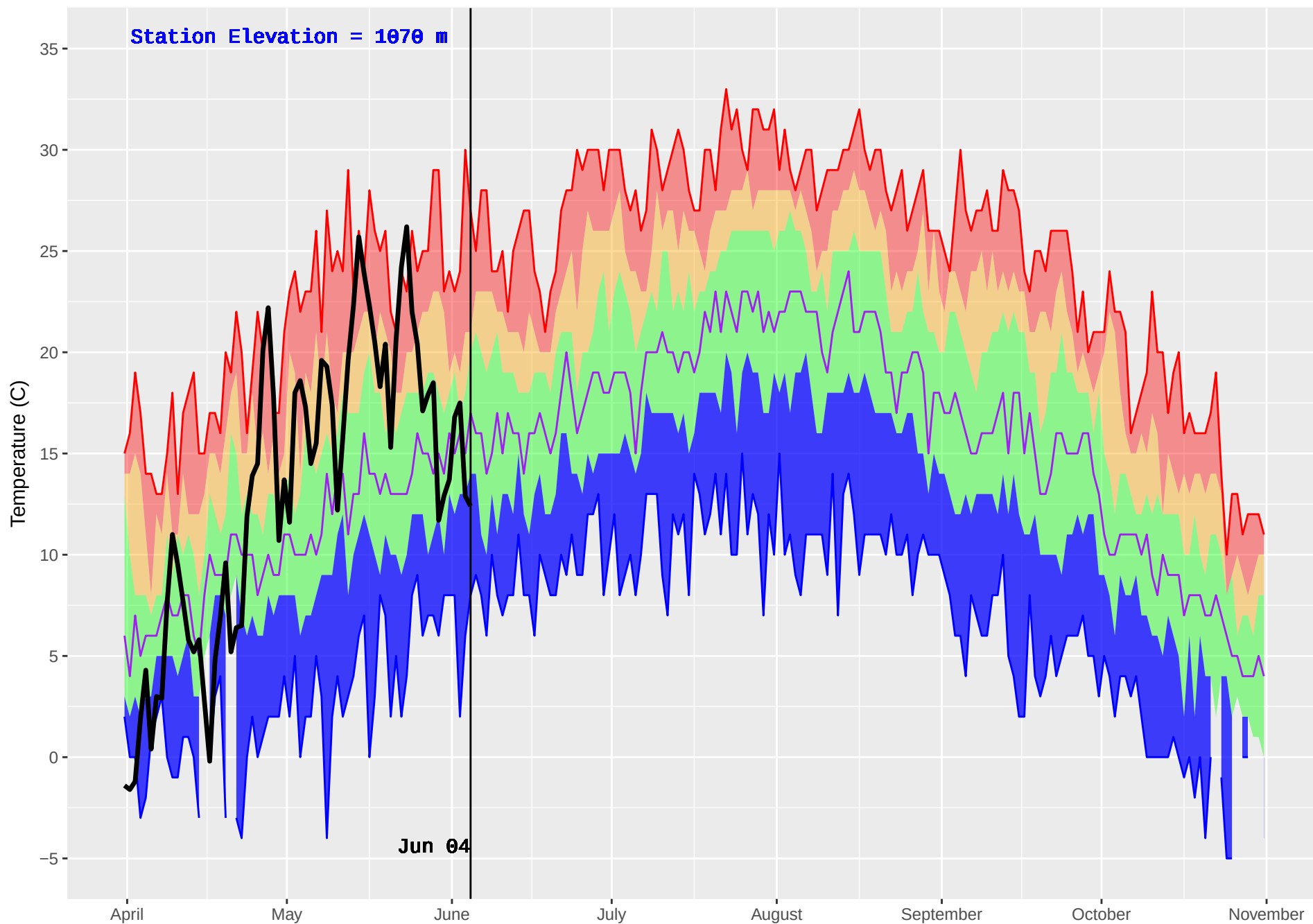
MEADOW LAKE (236) : Historical (1991–2016) and Current (2018) Noon Temperature
