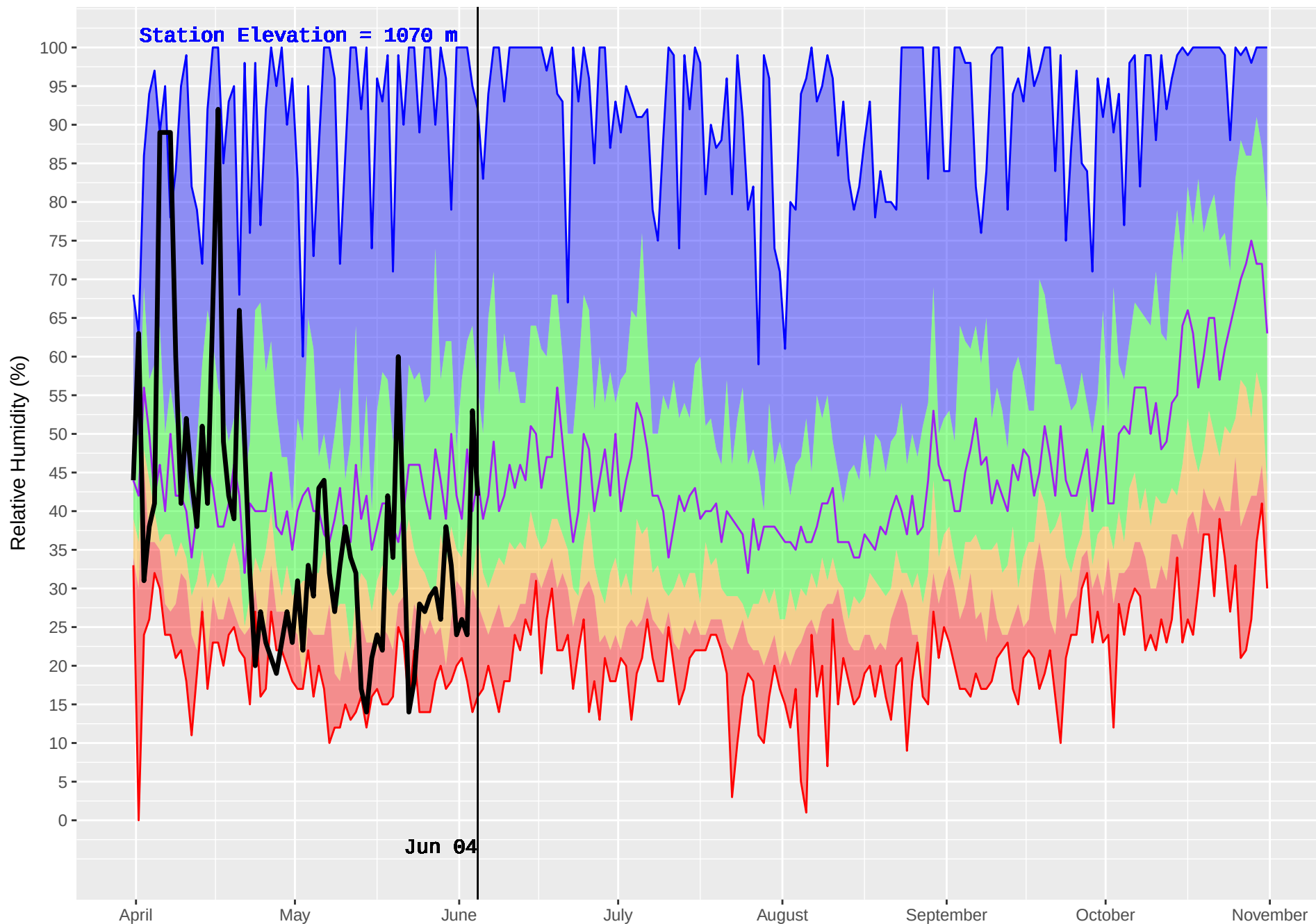
MEADOW LAKE (236) : Historical (1991–2016) and Current (2018) Noon Relative Humidity
