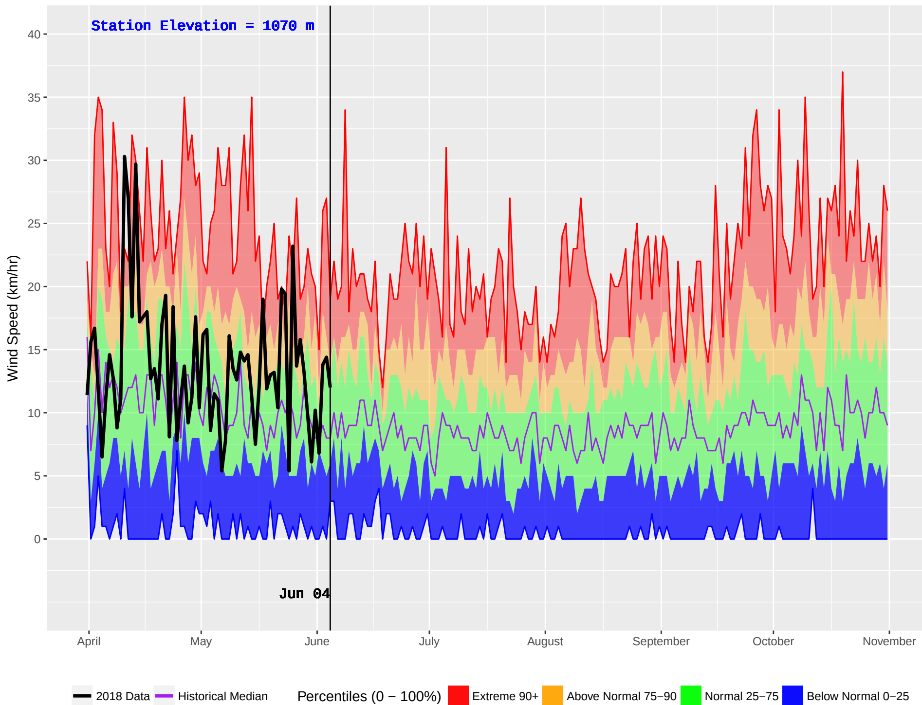
MEADOW LAKE (236) : Historical (1991–2016) and Current (2018) Noon Wind Speed
