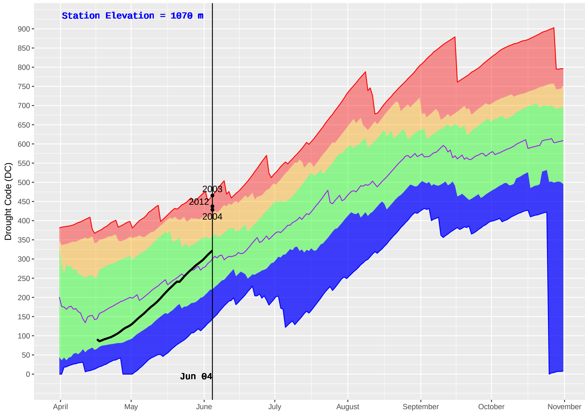
MEADOW LAKE (236) : Historical (1991–2016) and Current (2018) Noon Drought Code (DC)
