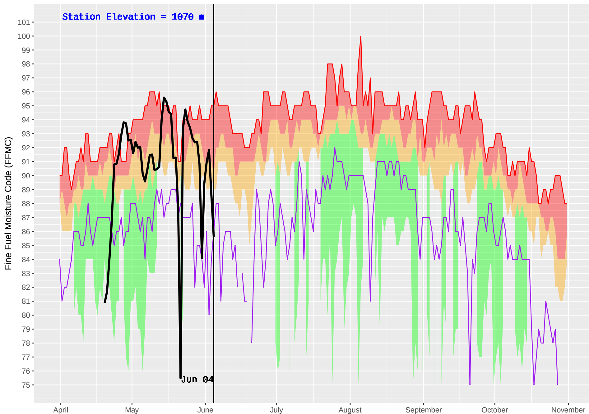
MEADOW LAKE (236) : Historical (1991–2016) and Current (2018) Noon Fine Fuel Moisture Code (FFMC)
